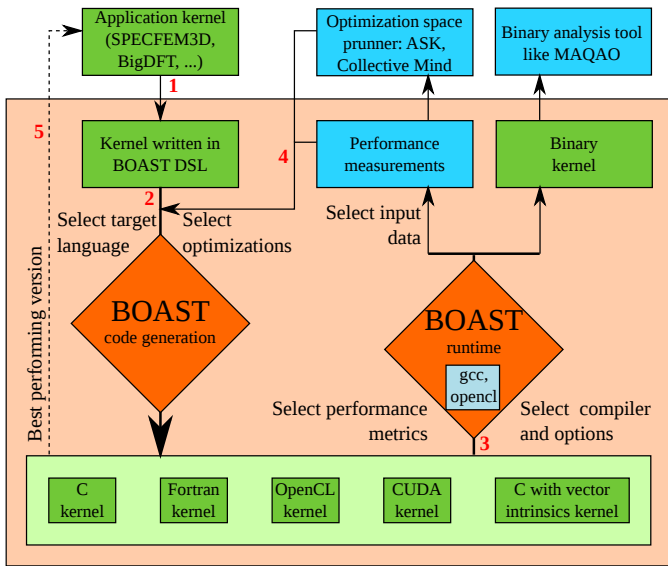
Fig. 1. Structure and Workflow of the BOAST framework.
