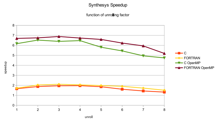
Fig. 5. Impact of Unrolling, Language Used and OpenMP on a Wavelet Transform Code.
