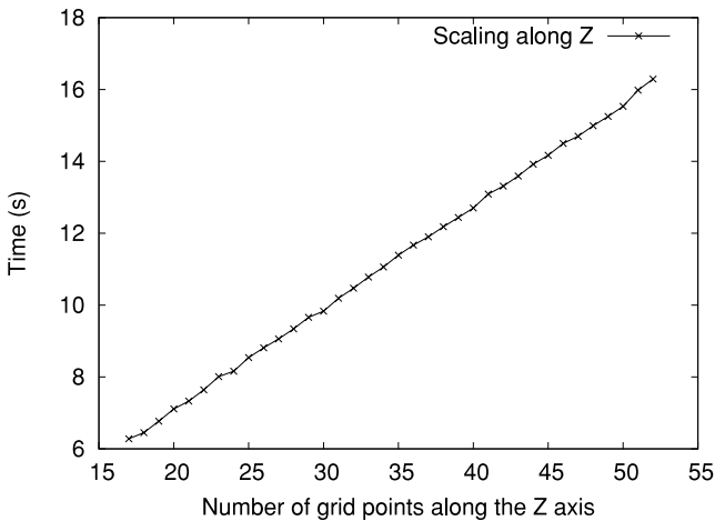
Figure 6. Strong scaling of the GPU 3-D finite-difference code running on a single GPU as a function of the number of points along Z , that is, variation of the total time spent running the code on the GPU when the number of gridpoints along the Z -axis of the grid increases. Scaling is almost linear, that is, almost perfect.
