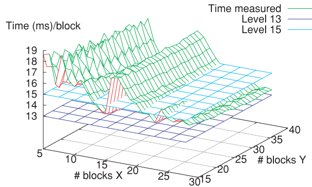
Figure 7. Scaling of the GPU 3-D finite-difference code running on a single GPU as a function of the number of thread blocks along the X - and Y -axes of the grid, that is, variation of the time spent by each block of threads to compute its share of the calculations on the GPU when the number of thread blocks varies. The size of each thread block and thus the number of calculations that it performs does not vary, therefore in an ideal case we should get a flat surface. Here, despite the coalesced memory accesses that we implemented, scaling along X is not regular and suffers from moderate variations that are likely due to undocumented hardware requirements. The blue and cyan horizontal planes indicate reference levels for comparison.
